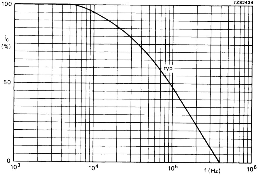
Fig. 13 I_B = 0 ; I_C = 2 mA; V_{CC} = 5 V; R_L = 1 k \Omega ; T_{amb} = 25 °C.
