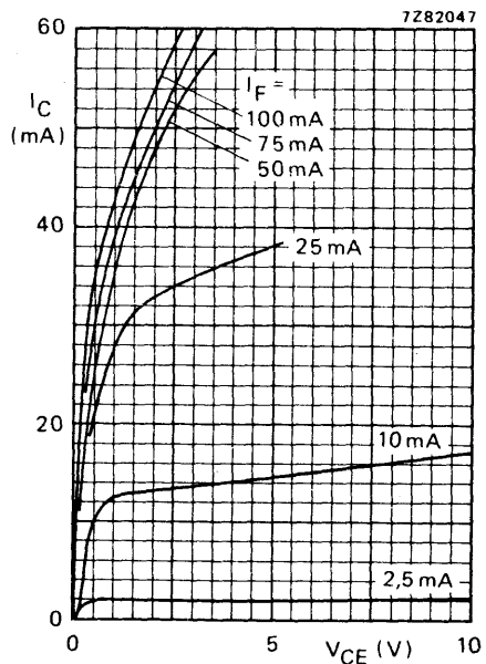
Fig. 16 CNY63; T_{amb} = 25 °C; typical values.
