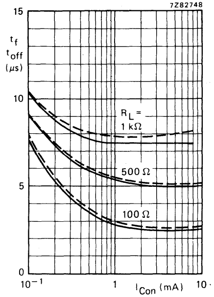
Fig. 12 — t_f ; --- t_{off} ; I_B = 0 ; V_{CC} = 20\ V ; T_{amb} = 25\ ^\circ C ; typical values. See also Fig. 13.
