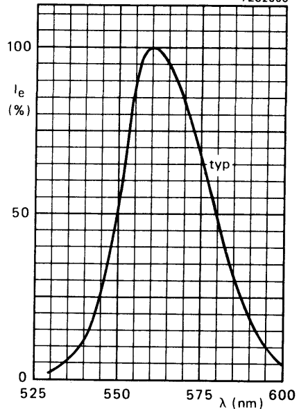
Fig. 9 CQX65 to 68.
