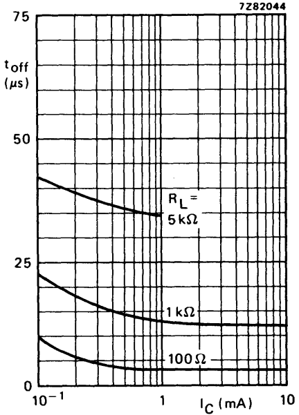
Fig. 20 CNY62; I_B = 0 ; V_{CC} = 5\text{ V} ; T_{amb} = 25\text{ }^\circ\text{C} ; typical values. (See also Fig. 21.)
