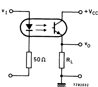
Fig. 3 Switching circuit.
