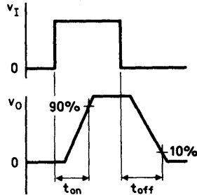
Fig. 21 Switching circuit and waveforms.
