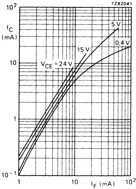
Fig. 13 CNY62; T_{amb} = 25 °C; typical values.
