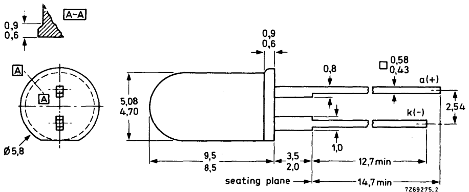
Fig. 1 SOD-63 (T-1%)
