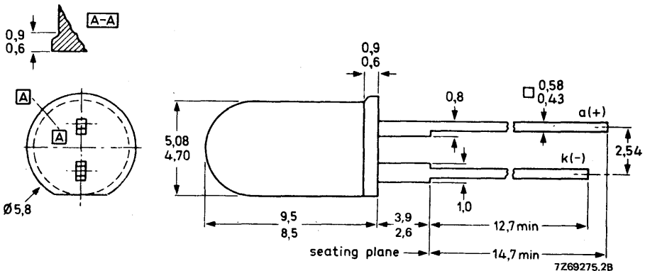
Fig.1 SOD-63 (except distance between base and seating plane), (T-1¼)
