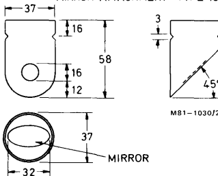
MIRROR ATTACHMENT - TYPE 13
