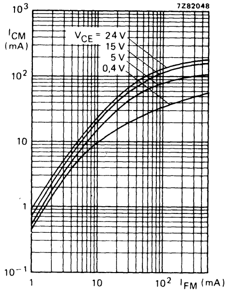
Fig. 14 CNY63; T_{amb} = 25 °C; t_p = 10 \mu s; T = 1 ms; typical values.
