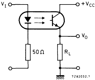
Fig. 2 Switching circuit.
