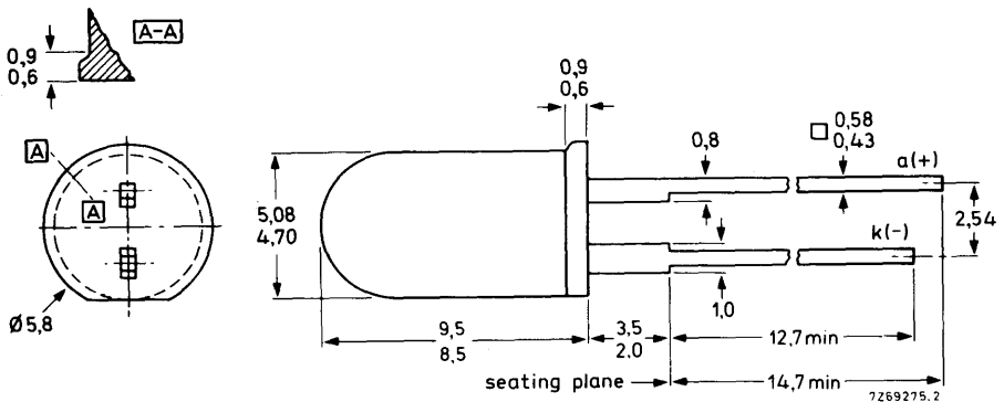
Fig.1 SOD-63 (T-1%)
