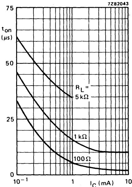
Fig. 19 CNY62; I_B = 0 ; V_{CC} = 5\text{ V} ; T_{amb} = 25\text{ }^\circ\text{C} ; typical values. (See also Fig. 21.)
