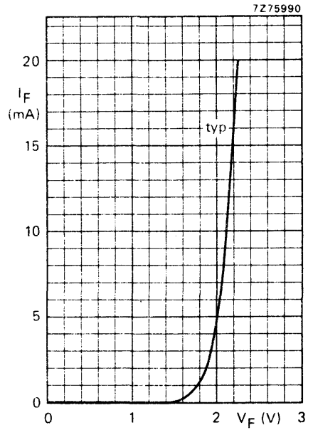
Fig. 6 T_j = 25 \text{ °C} .
