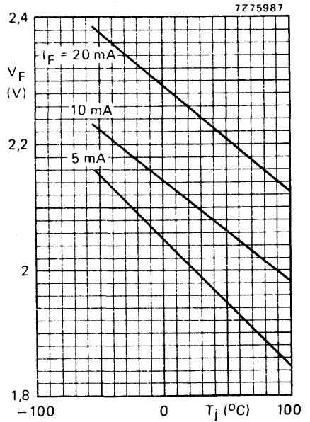
Fig. 8 Typical values.
