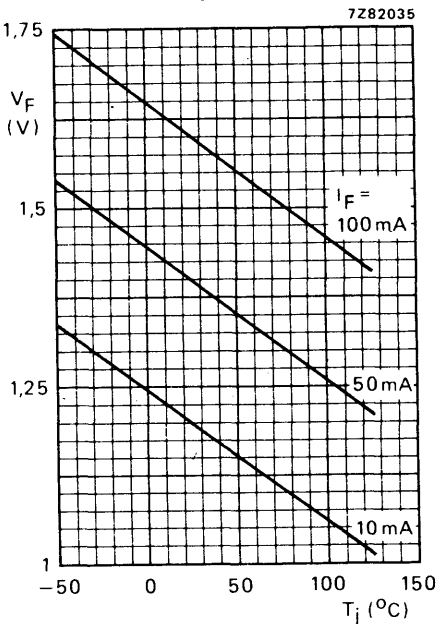
Fig. 7 Typical values.
