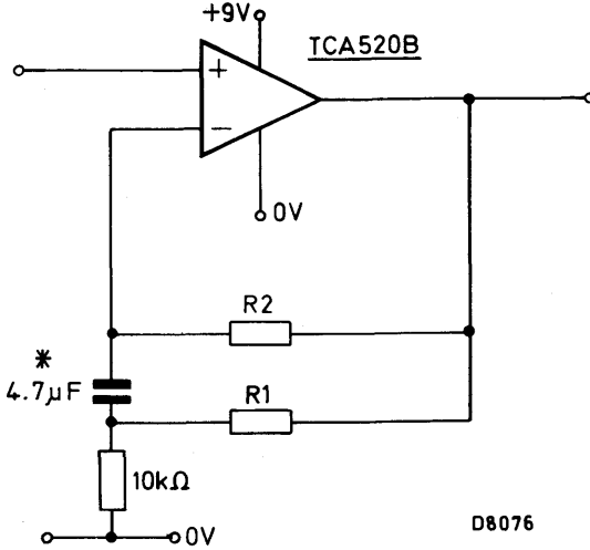
Recommended component values for various gains
