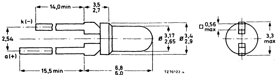
Fig. 1 SOD-53C (T-1)
