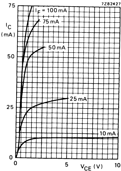
Fig. 14 T_{amb} = 25 °C; typical values.
