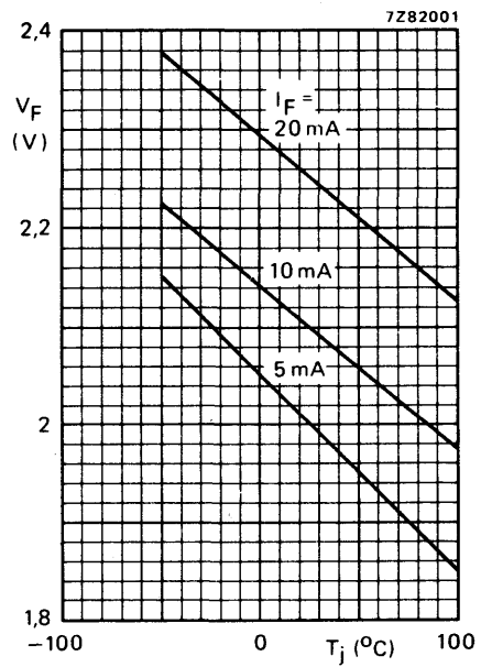
Fig. 4 Typical values.
