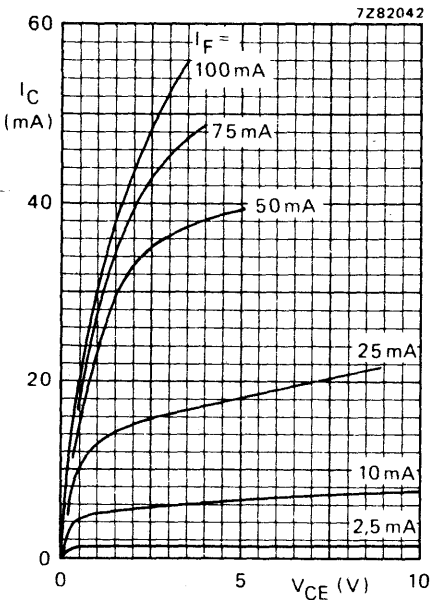
Fig. 15 CNY62; T_{amb} = 25 °C; typical values.
