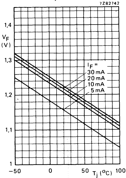
Fig. 7 Typical values.
