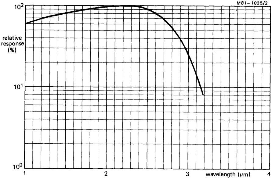
Typical spectral response at 20 °C
