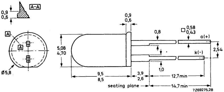
Fig. 1 SOD-63 (except distance between base and seating plane). (T-1%)
