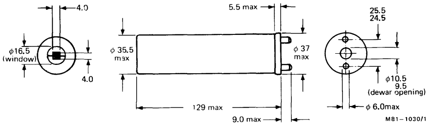
MIRROR ATTACHMENT - TYPE 13
