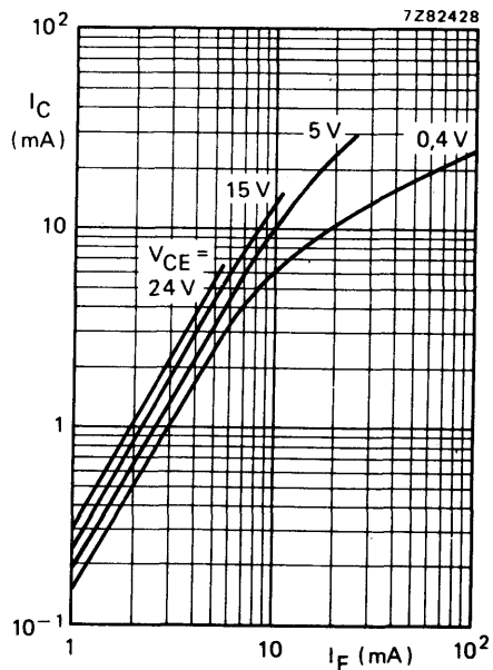
Fig. 15 T_{amb} = 25 °C; typical values.
