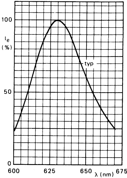
Fig. 8 CQX55 to 58.
