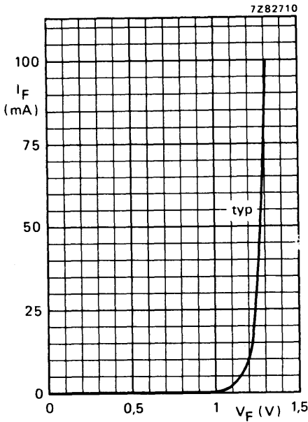
Fig. 5 T_{amb} = 25^{\circ}C .
