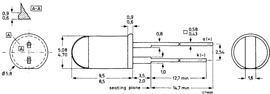
Fig. 1d SOD-63M applicable to CQX58/68/78.
