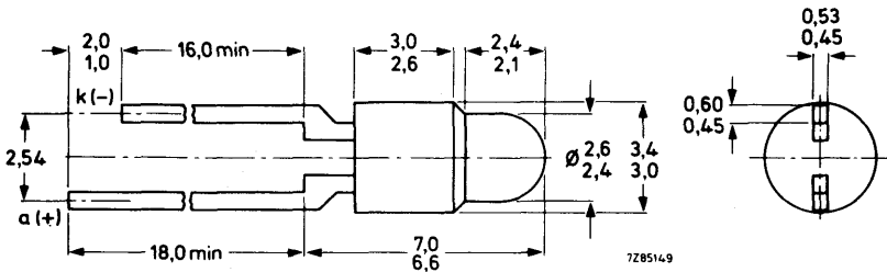
Fig. 1 SOD-53D (T-1)
