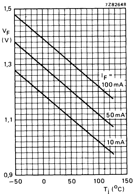
Fig. 7 Typical values.
