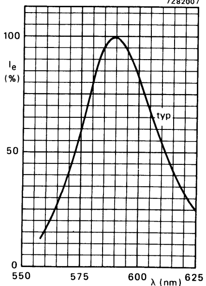
Fig. 10 CQX75 to 78.
