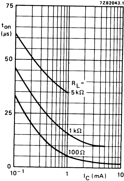
Fig. 23 I_B = 0 ; V_{CC} = 5\text{ V} ; T_{amb} = 25\text{ }^\circ\text{C} ; typical values. (See also Fig. 25.)
