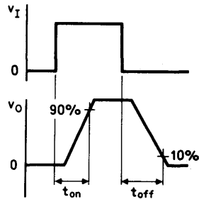
Fig. 4 Waveforms.
