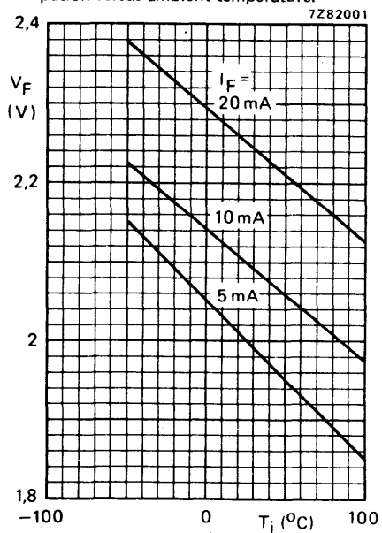
Fig. 4 Typical values.
